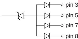
Circuit of ALC inputs (pin 3, 5, 7, and 8)
