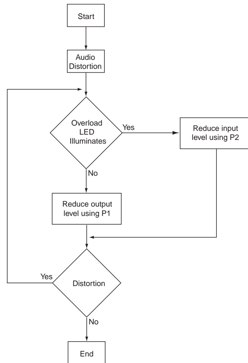
Figure 6. Troubleshooting flowchart.
