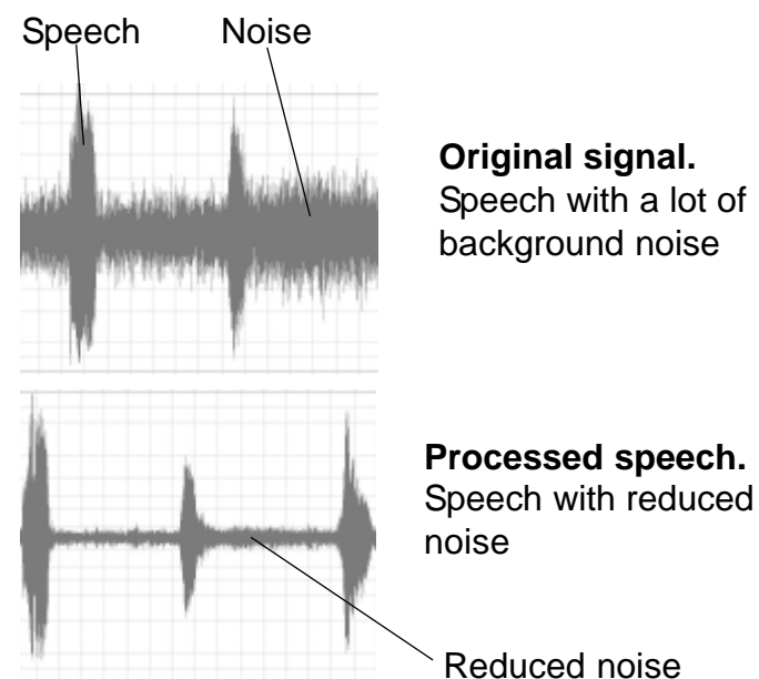
Figure 1. Noise cancellation.
